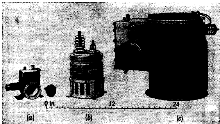
FIG. 13-11.—Three pulse transformers designed for operation at different power levels. (a) 120 kw (232 BW2) with well for magnetron (Westinghouse). (b) 2 Mw (GE) (c) 10 Mw (377 BW2) with form-fitting well for magnetron (GE).
